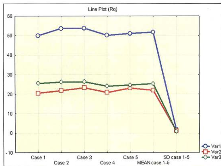
Fig. 8. Graphic representation of the profilometric data (reports in Table 2) on each surface of the absolute values of the root-mean-square of the values of all point ( R_q ). (Var1: Sab; Var2: SLA; Var3: FCC).
