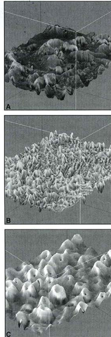
Fig. 10. StereoSEM 3D reconstruction of the 3 different implant surface. (A: Sab; B: SLA; C: FCC). FCC implant microroughness, due to the specific electrochemical treatment, resulted more homogeneous than the one recorded for the Sab and SLA implant groups.
