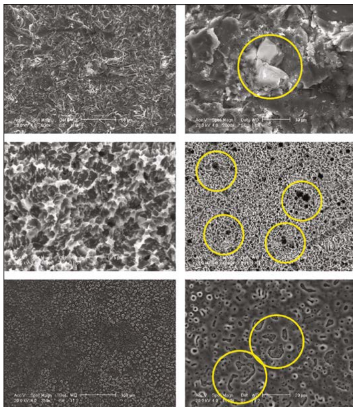
Fig. 6A. Upper panel: SEM and EDAX analysis of SAB implant surface. Middle panel: SEM and EDAX analysis of SLA implant surface. Lower panel: SEM and EDAX analysis of FCC implant surface.
