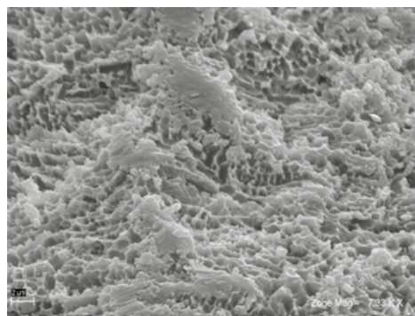
Figure 8B - SEM visualization of the Micro Rough Surface® at higher magnification (A:1980x; B: 7330x).
