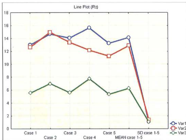
Fig. 9. Graphic representation of the profilometric data (reported in Table 3) on each surface of the absolute height of the 5 highest peaks and the absolute depth of the 5 deepest valleys ( R_z ). (Var1: Sab; Var2: SLA; Var3: FCC).
