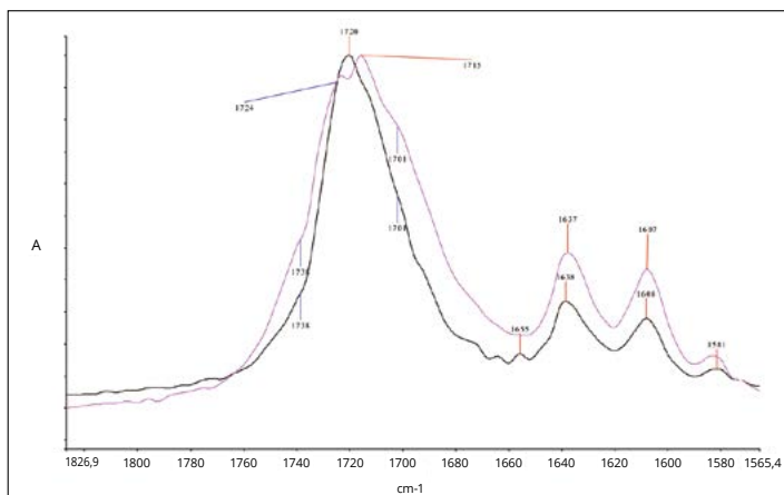
Figure 3.—Splitting of the carbonyl band.
