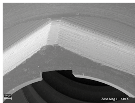
Figure 4 - SEM visualization of the machined neck surface (149x magnification).
