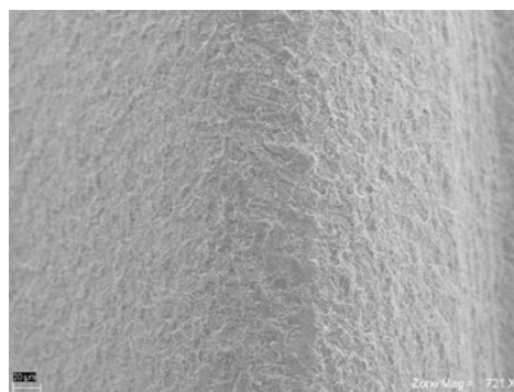
Figure 7 - SEM visualization of the Micro Rough Surface® regularly distributed (721x magnification).
